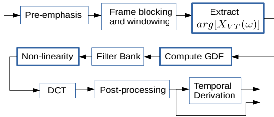
Fig. 2. Phase filter-based feature extraction proposed in [18].
