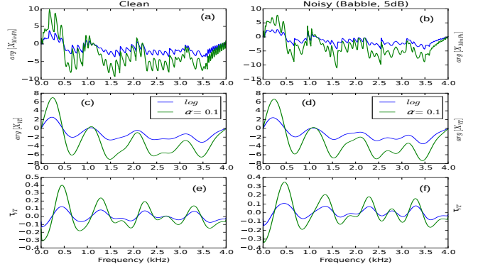
Fig. 3. Effect of using GenLog(|X|) in the Hilbert Transform at the clean and noisy (Babble, 5 dB) conditions. (a) arg[X_{MinPh}] -clean, (b) arg[X_{MinPh}] -noisy, (c) arg[X_{VT}] -clean, (d) arg[X_{VT}] -noisy (e), \tau_{VT} -clean, (f) \tau_{VT} -noisy.
