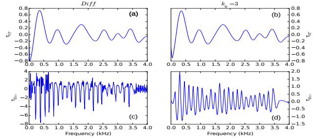
Fig. 4. Sample difference (Diff) vs regression filter for computing the derivatives of filter and source GDs ( \alpha = 0.1 ). (a) \tau_{VT}[Diff] , (b) \tau_{VT}[k_0 = 3] , (c) \tau_{Exc}[Diff] , (d) \tau_{Exc}[k_0 = 3] .
