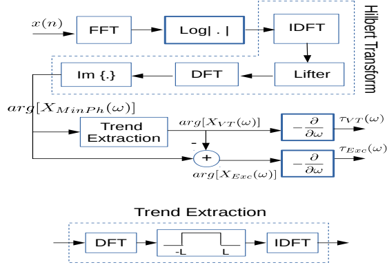
Fig. 1. Phase-based source-filter decomposition proposed in [18].
