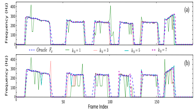
Fig. 5. Effect of k_0 on the accuracy/robustness of phase-based F_0 estimation using (9) for sb003.sig from [25] ( \alpha = 0.1 ). (a) clean, (b) noisy (White, 5 dB). No post-processing on F_0 has been applied.
